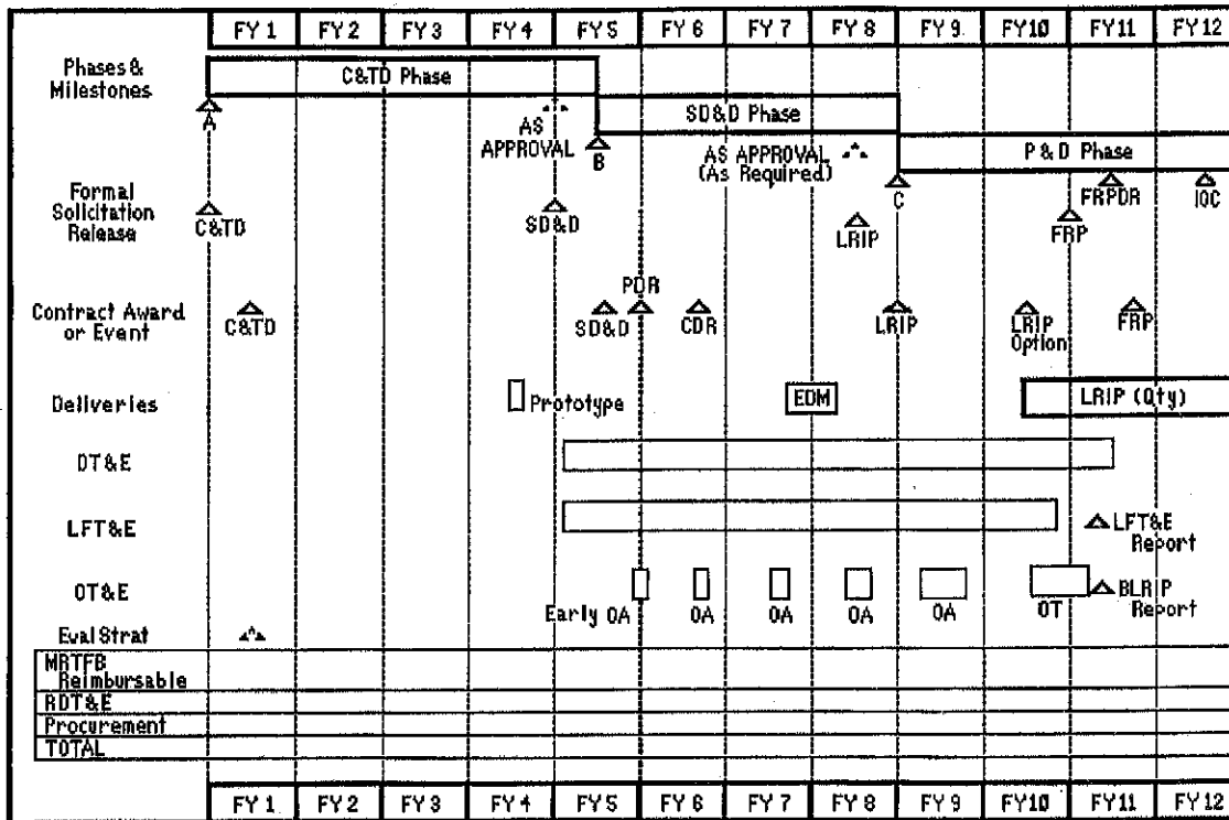
AP2.F1. Figure 1 -- Integrated Test Program Schedule
